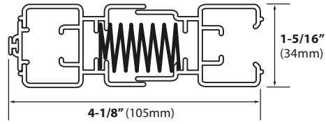
SCREEN PANEL PROFILES WITH PLEATED FABRIC
